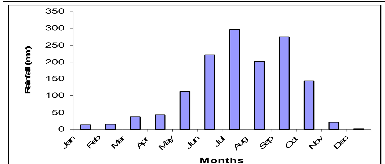
Mean monthly rainfall of Nadia district
